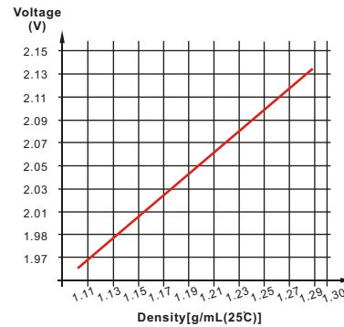
Electrolyte Density in Relation to Voltage
