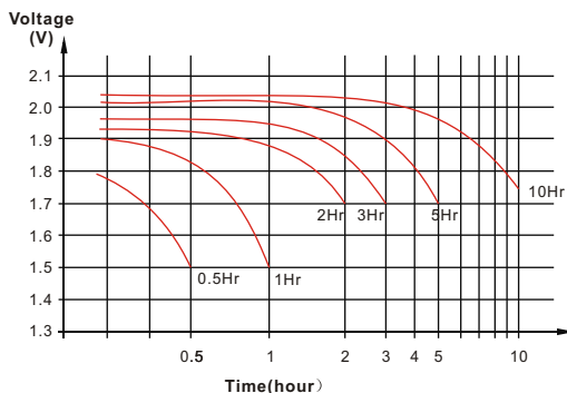
Discharge Characteristics
